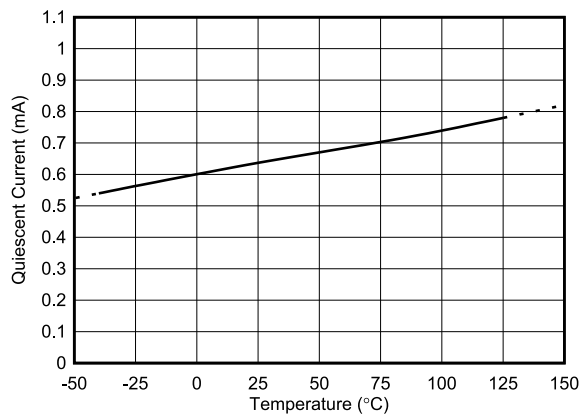
Figure 5-16. Active I_Q vs Temperature
