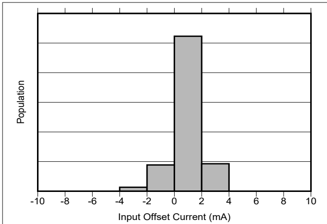
Figure 5-2. Shunt Input Offset Current Production Distribution
