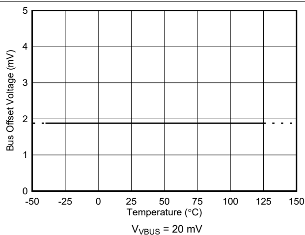
Figure 5-10. Bus Input Offset Voltage vs Temperature
