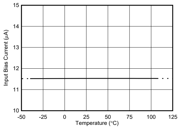
Figure 5-14. Input Bias Current ( I_{B^+} + I_{B^-} ) vs Temperature
