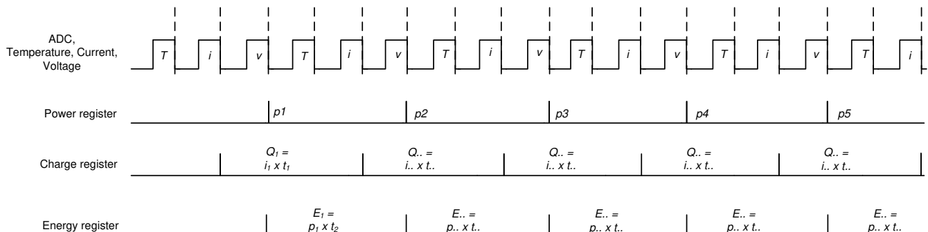
Figure 6-6. Power, Energy, and Charge Calculation Scheme
