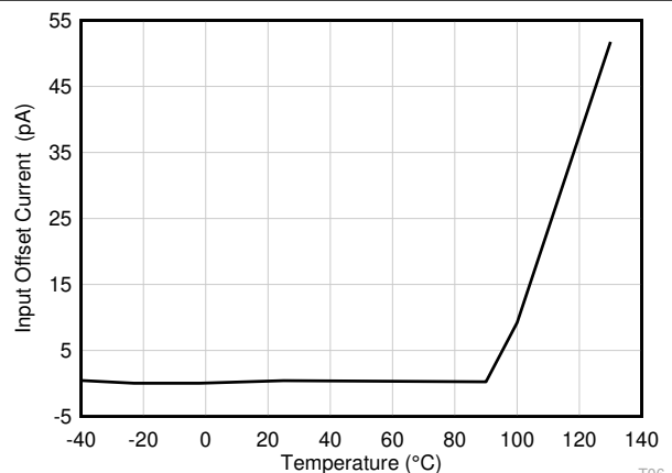
Figure 7-11. Input Offset Current vs Temperature
