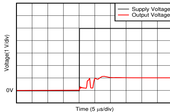
Figure 6-32. Start-Up Response
