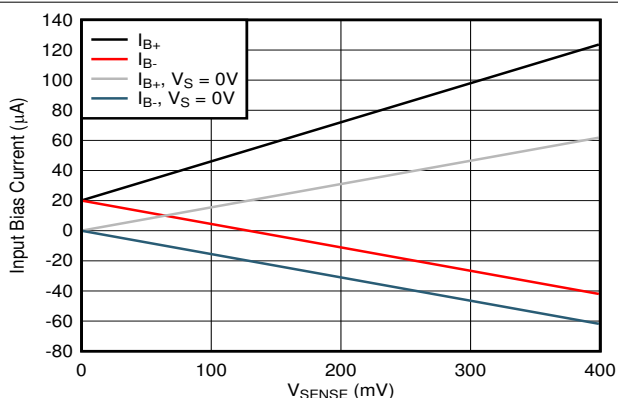
Figure 6-16. INA310x2-Q1, INA310x3-Q1 Input Bias Current vs V_{SENSE}
