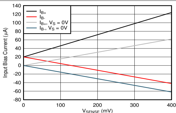
Figure 6-16. INA310x2, INA310x3 Input Bias Current vs V_{SENSE}
