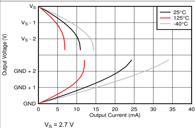
Figure 6-18. Output Voltage vs Output Current
