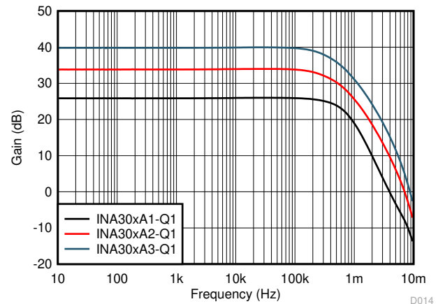
Figure 6-14. Gain vs. Frequency
