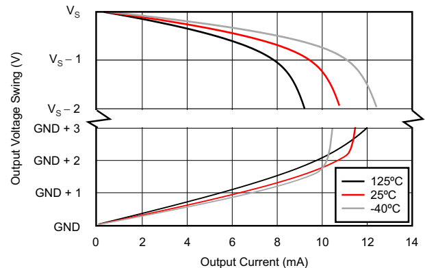
Figure 6-16. Output Voltage Swing vs. Output Current
