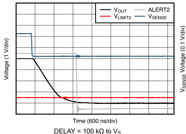
Figure 6-33. Comparator 2 Total Propagation Delay (INA303-Q1)
