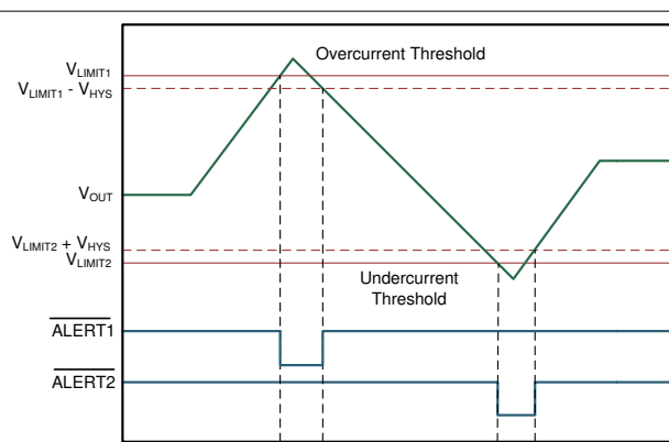
Figure 7-5. Comparator Hysteresis Behavior (INA303-Q1)
