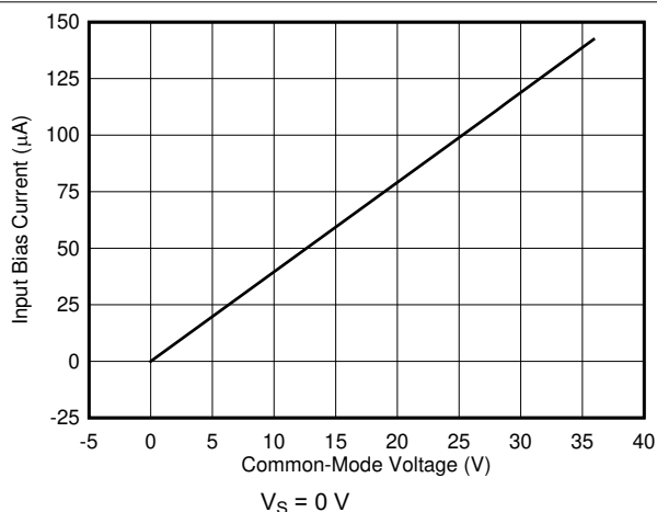
Figure 6-18. Input Bias Current vs. Common-Mode Voltage
