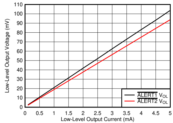
Figure 6-38. Comparator Alert V_{\text{OL}} vs. I_{\text{OL}}
