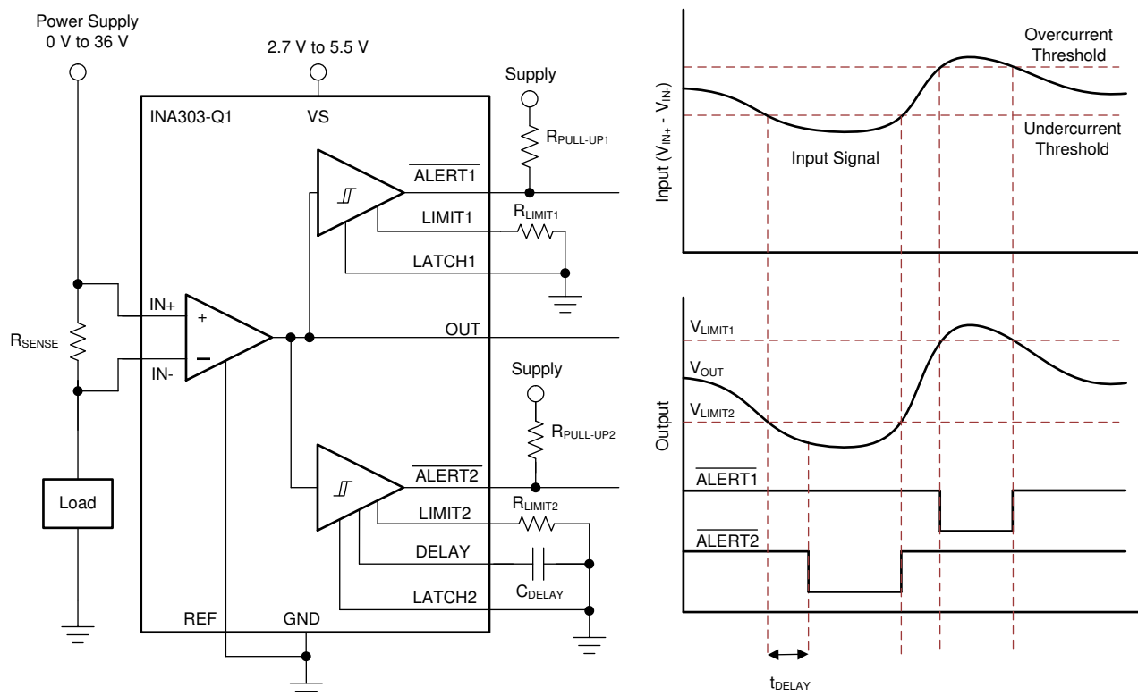
Figure 7-2. Out-of-Range Alert Responses for the INA303-Q1
