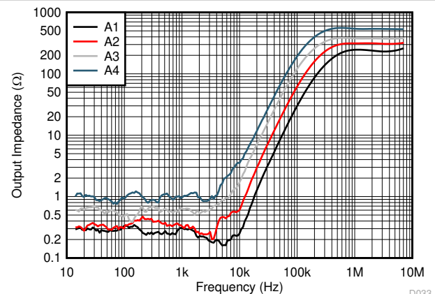
Figure 6-42. Output Impedance vs. Frequency
