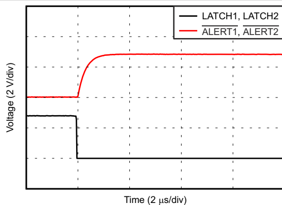
Figure 6-41. Comparator Latch Response
