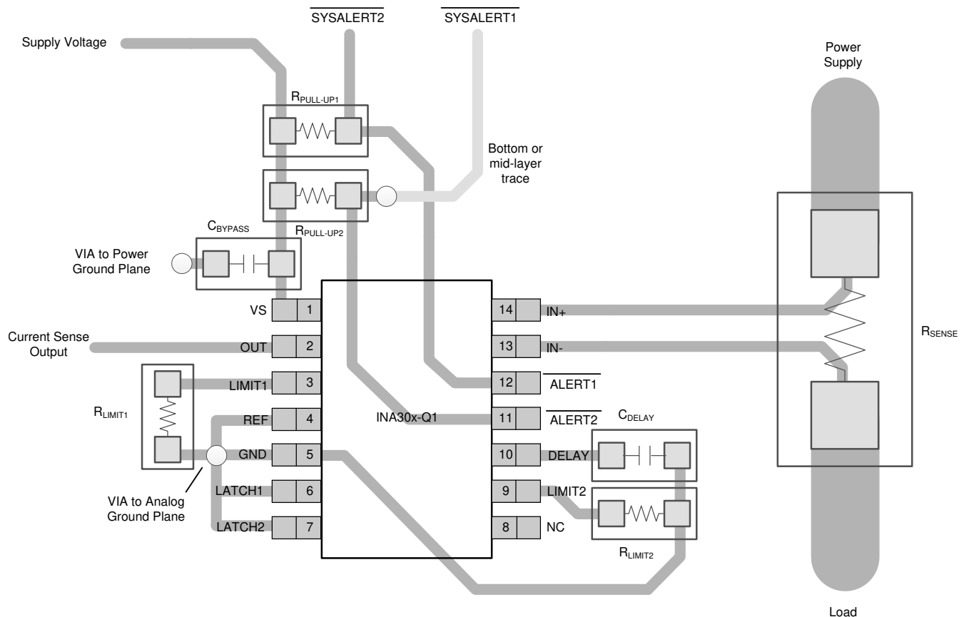
Figure 10-1. Recommended Layout
