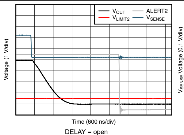
Figure 6-32. Comparator 2 Total Propagation Delay (INA303-Q1)
