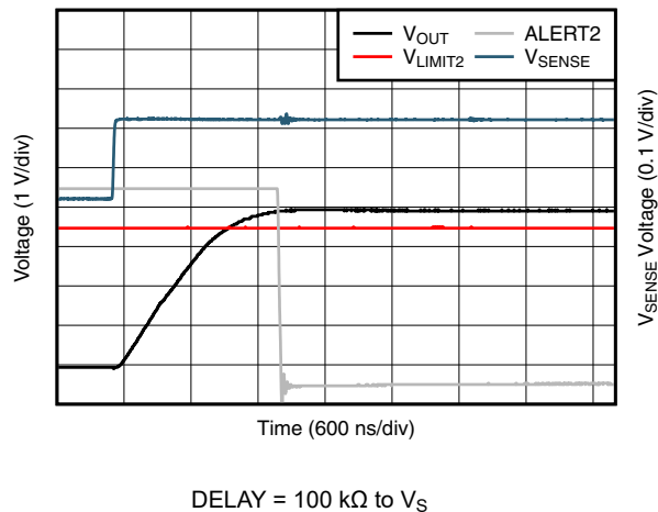
Figure 6-35. Comparator 2 Total Propagation Delay (INA302-Q1)
