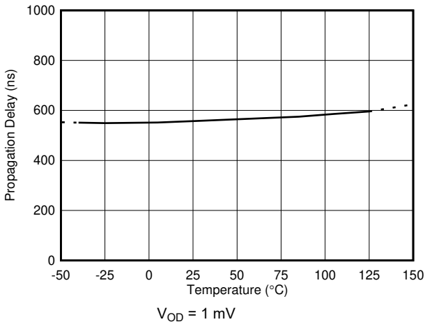
Figure 6-36. Comparator 1 Propagation Delay vs. Temperature
