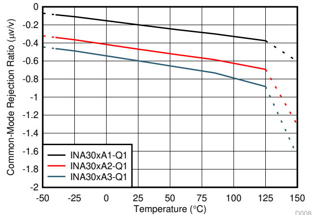
Figure 6-8. CMRR vs. Temperature
