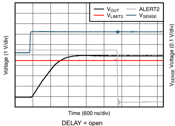
Figure 6-34. Comparator 2 Total Propagation Delay (INA302-Q1)
