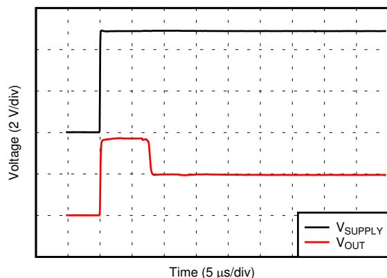
Figure 6-27. Start-Up Response
