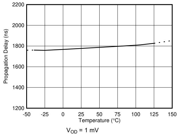
Figure 6-37. Comparator 2 Propagation Delay vs. Temperature
