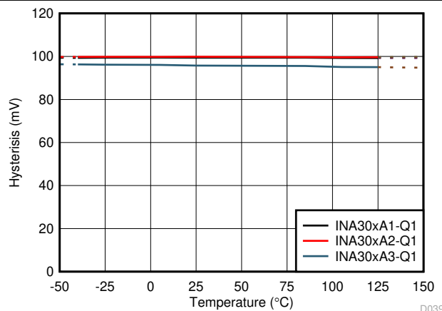
Figure 6-39. Comparator 1 Hysteresis vs. Temperature
