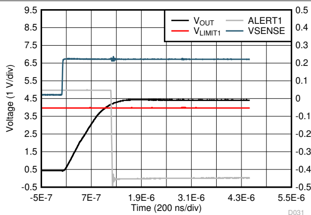
Figure 6-31. Comparator 1 Total Propagation Delay (INA30x-Q1)
