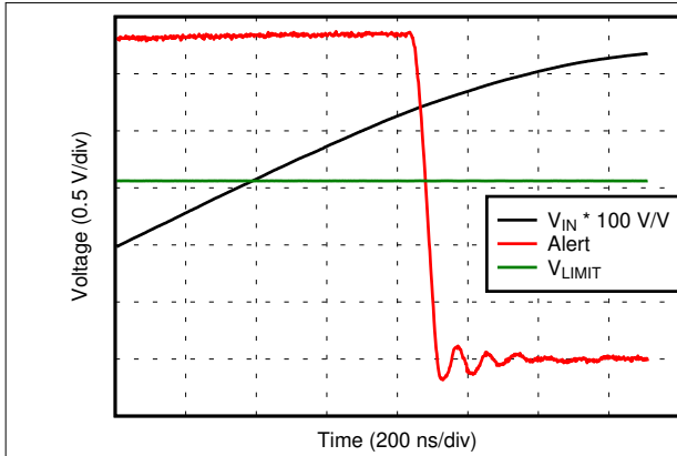
Figure 6-31. Total Propagation Delay (INA301A3-Q1)
