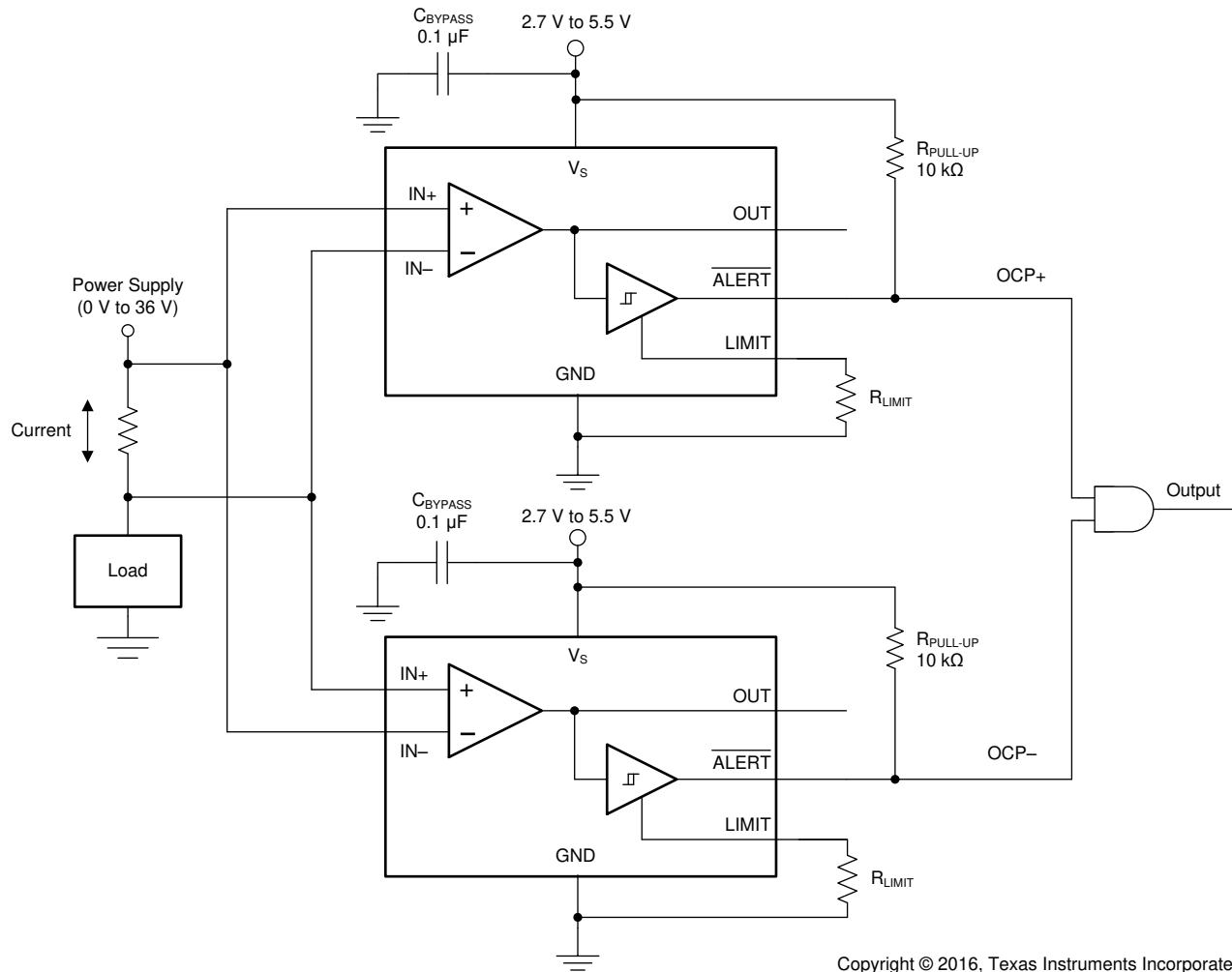
Figure 8-4. Bidirectional Application
