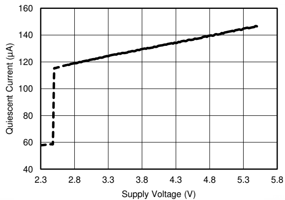
Figure 6-11. Quiescent Current vs Supply Voltage (Enabled)
