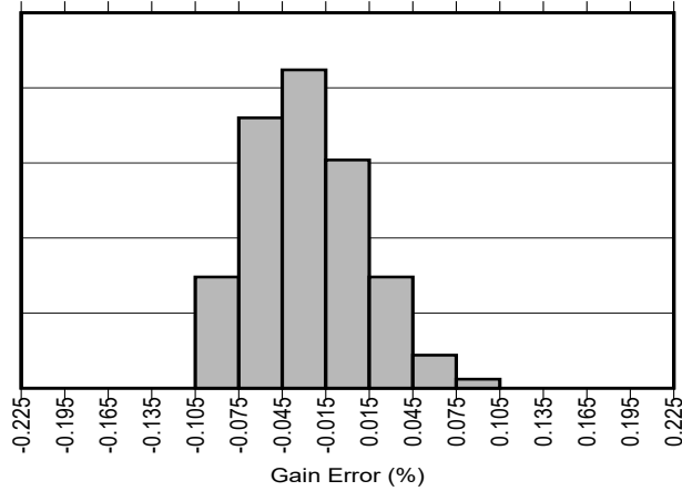
Figure 5-7. INA299-Q1 Gain Error Production Distribution
