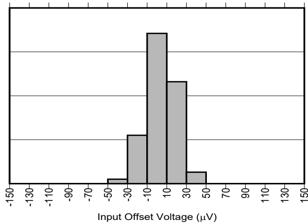
Figure 5-1. INA299-Q1 Input Offset Voltage Production Distribution
