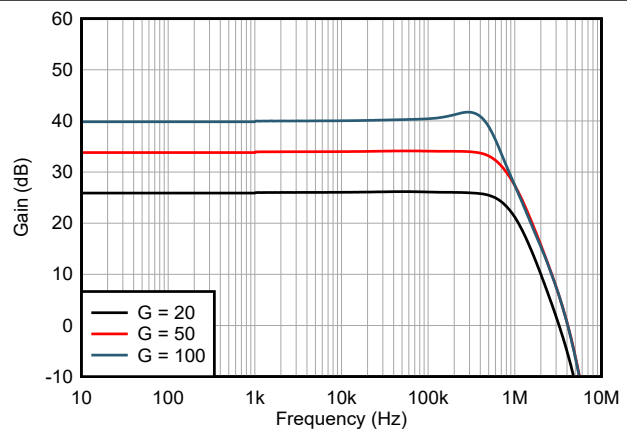
Figure 5-6. Gain vs Frequency
