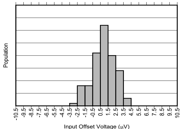
Figure 6-2. INA296A2-Q1 Input Offset Production Distribution
