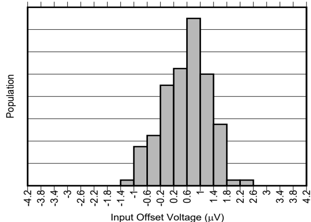
Figure 6-4. INA296A5-Q1 Input Offset Production Distribution
