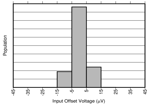
Figure 6-3. INA293x3 Input Offset Production Distribution
