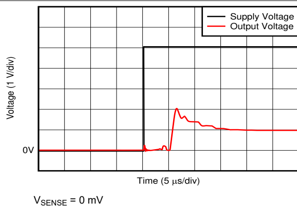
Figure 6-33. Start-Up Response
