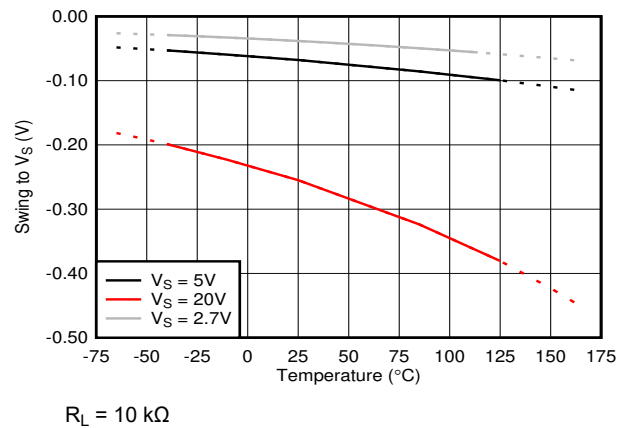
Figure 6-22. Swing to Supply vs Temperature
