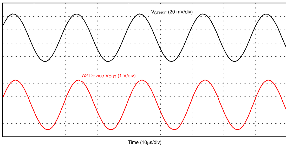
Figure 8-3. INA280 Output Response
