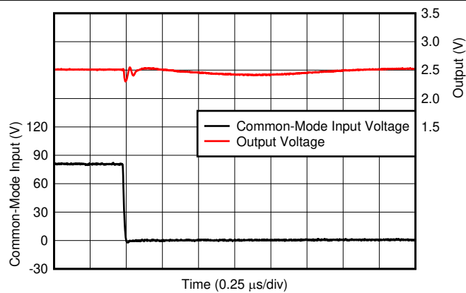
Figure 7-31. Common-Mode Voltage Transient Response
