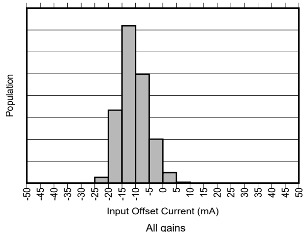
Figure 7-1. Input Offset Current Production Distribution
