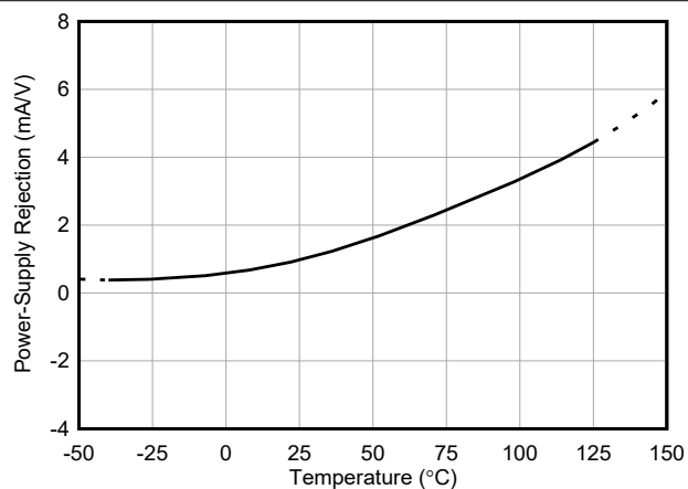
Figure 7-5. Power-Supply Rejection Ratio vs Temperature
