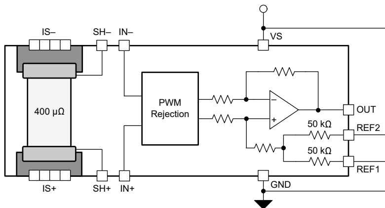
Figure 8-8. Mid-Supply Voltage Output
