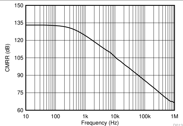
Figure 7-12. Common-Mode Rejection Ratio vs Frequency
