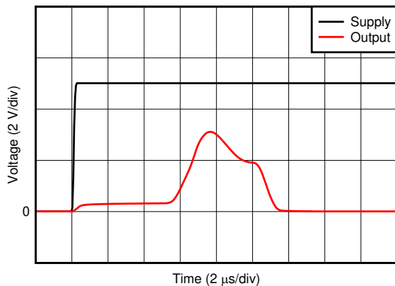
Figure 7-27. Amplifier Step Response
