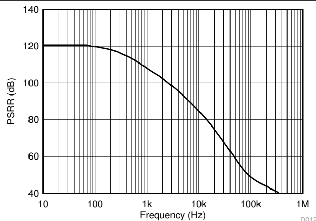
Figure 7-11. Power-Supply Rejection Ratio vs Frequency
