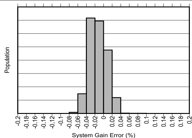
Figure 7-6. Gain Error Production Distribution (INA254A1)
