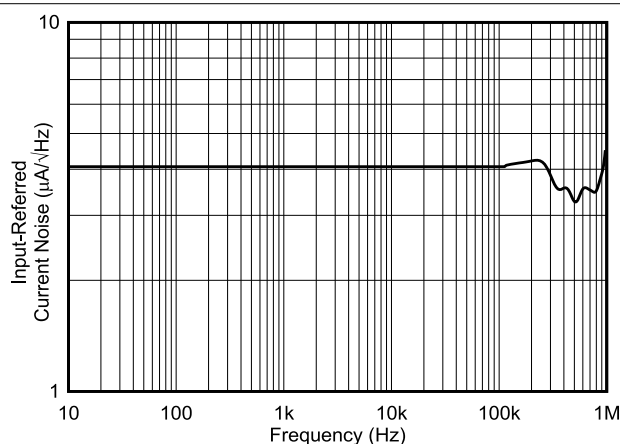
Figure 7-23. INA254A1 Input-Referred Current Noise vs Frequency
