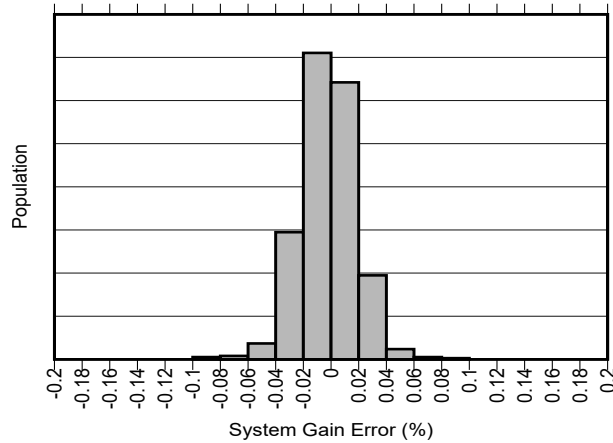
Figure 7-7. Gain Error Production Distribution (INA254A2)
