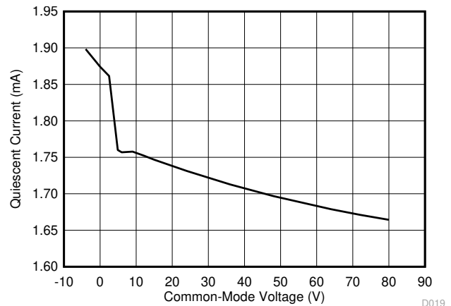
Figure 7-22. Quiescent Current vs Common-Mode Voltage
