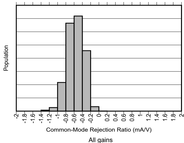
Figure 7-3. Common-Mode Rejection Production Distribution
