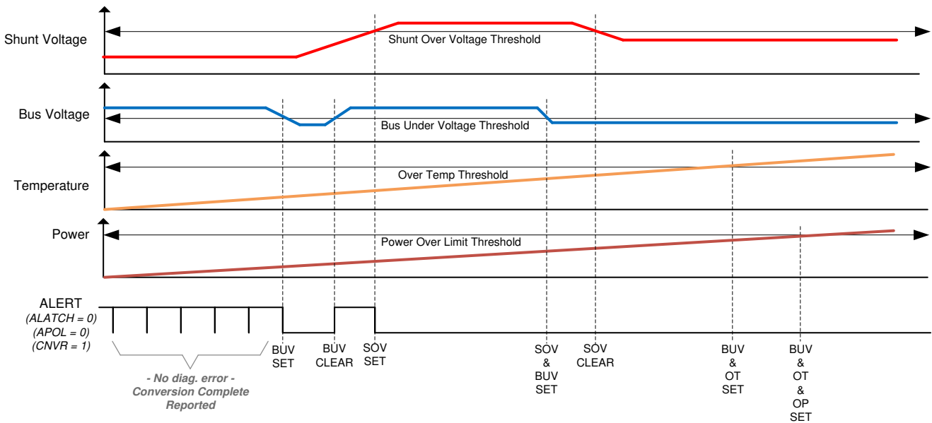
Figure 6-6. Multi-Alert Configuration
