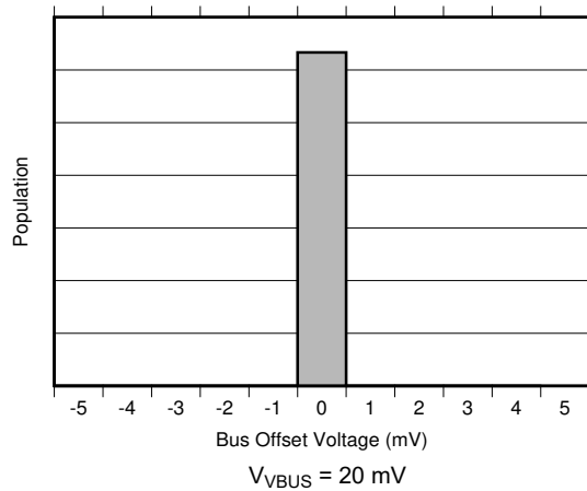
Figure 5-10. Bus Input Offset Voltage Production Distribution
