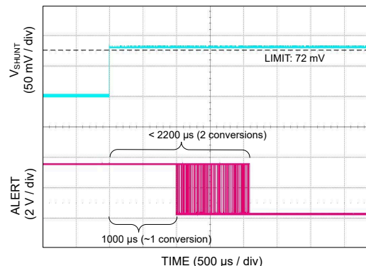
Figure 8-4. Alert Response ( t_{CT} = 1.1 ms )
