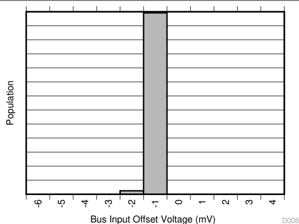
Figure 5-8. Bus Input Offset Voltage Production Distribution
