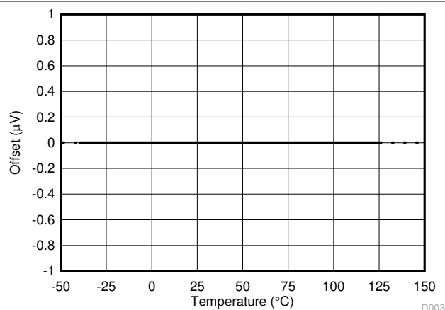
Figure 5-3. Shunt Input Offset Voltage vs Temperature
