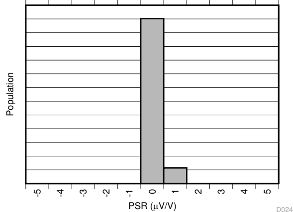
Figure 5-15. Power-Supply Rejection Distribution
