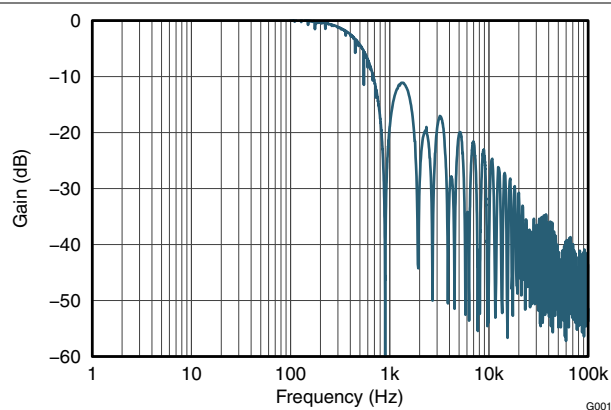
Figure 5-1. Frequency Response
