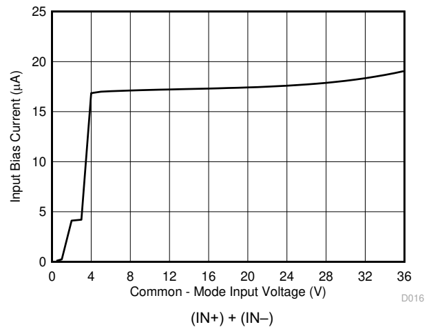
Figure 5-16. Input Bias Current vs Common-Mode Voltage
