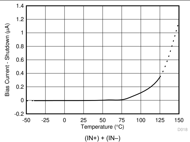
Figure 5-18. Input Bias Shutdown Current vs Temperature
