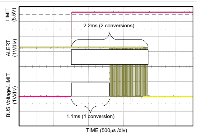
Figure 7-3. Alert Response ( t_{CT} = 1.1ms )
