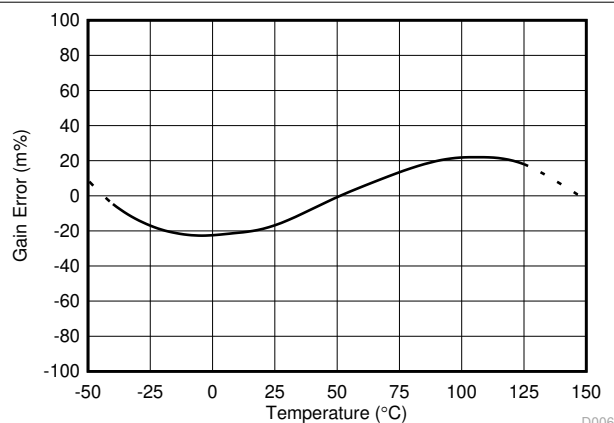
Figure 5-6. Shunt Input Gain Error vs Temperature
