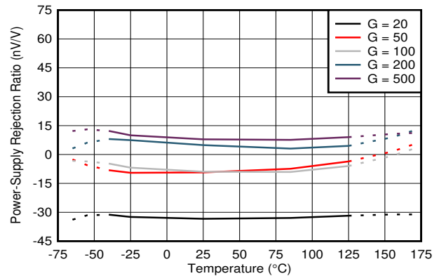
Figure 6-12. Power-Supply Rejection Ratio vs. Temperature
