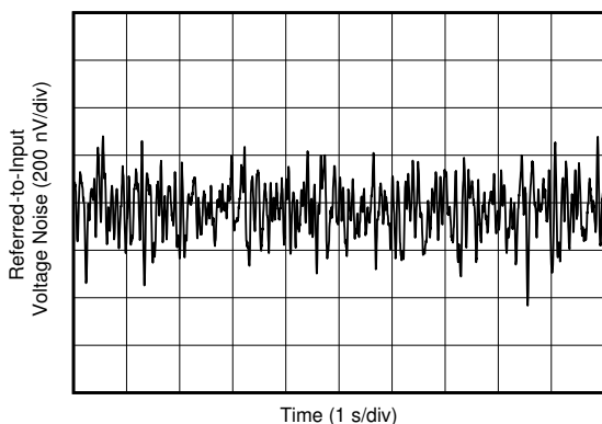
Figure 6-27. Input-Referred Noise
