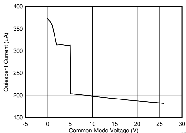
Figure 6-26. I_Q vs Common-Mode Voltage (INA181)
