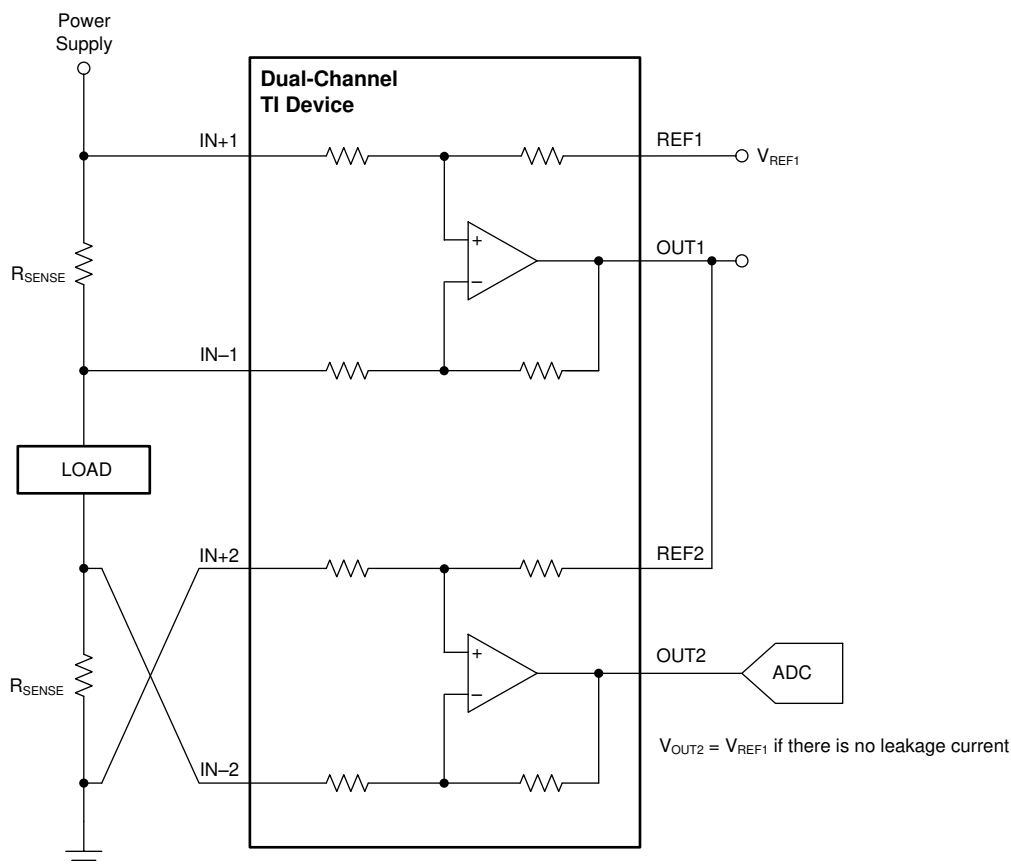
Figure 8-5. Detecting Leakage Currents
