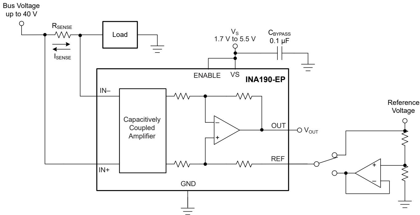
Figure 7-4. Bidirectional Application
