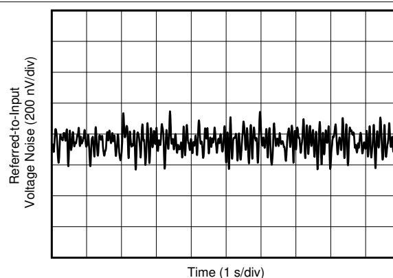
Figure 7-30. 0.1-Hz to 10-Hz Voltage Noise (Referred-to-Input)
