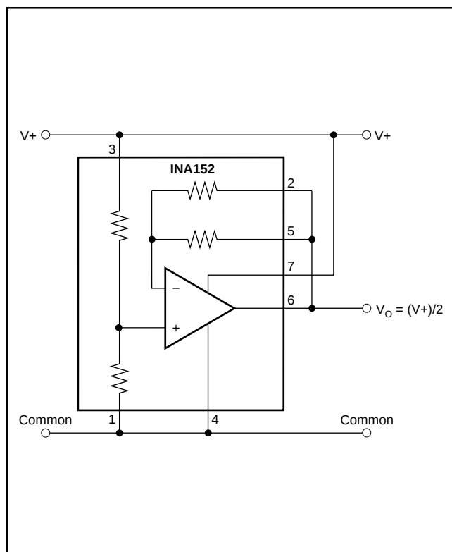
FIGURE 5. Pseudoground Generator.
