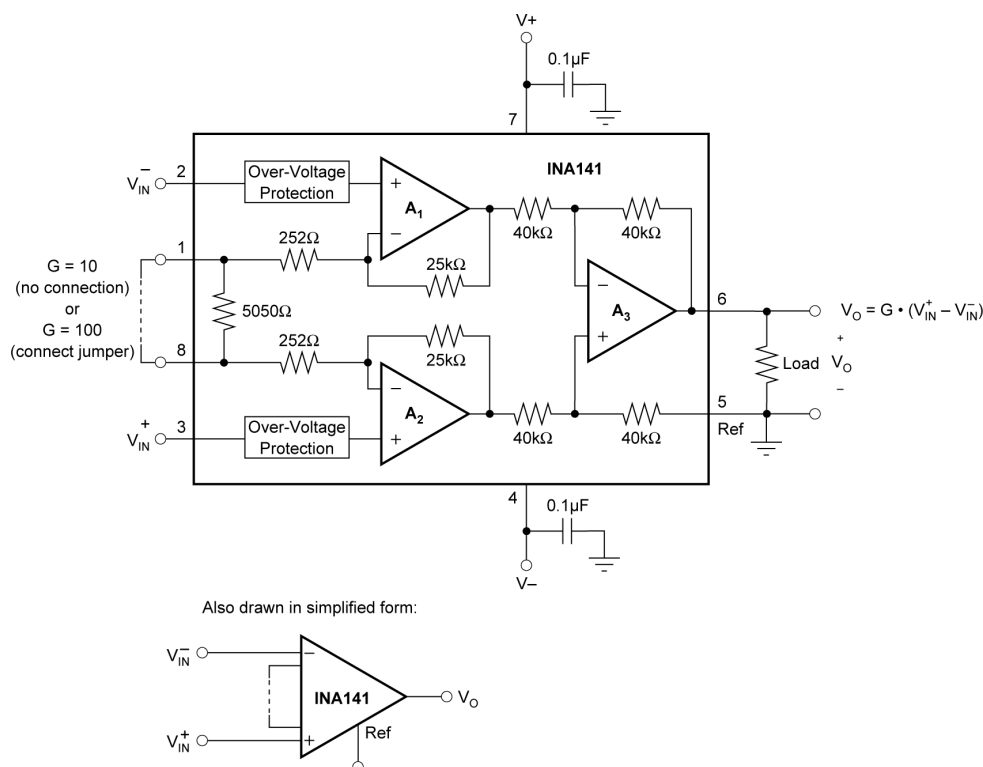
Figure 7-1. Basic Connections.
