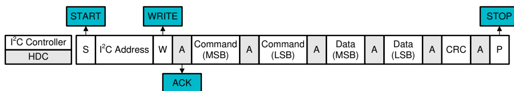
Figure 7-2. I 2 C Write Command, Configuration Data and CRC Byte Required
