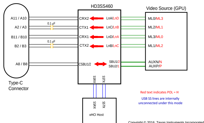
Figure 8. SOURCE Pin Assignment Option C and E (AMSEL = H, EN = H)
