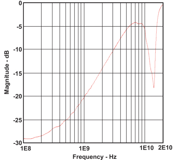
Figure 9-6. Return Loss
