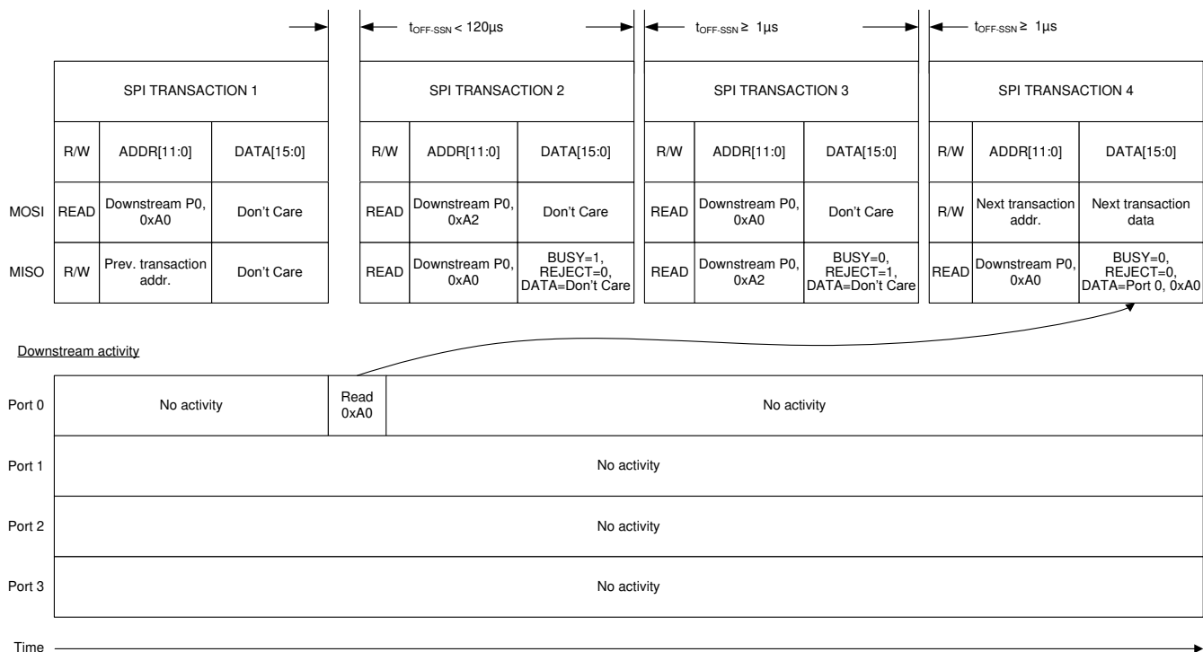
Figure 8-11. Back-to-Back SPI Reads From Same Port
