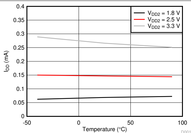
Figure 7-3. Static IDD2 vs. Ambient Temperature
