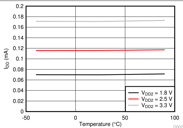
Figure 7-4. Dynamic IDD2 vs. Ambient Temperature
