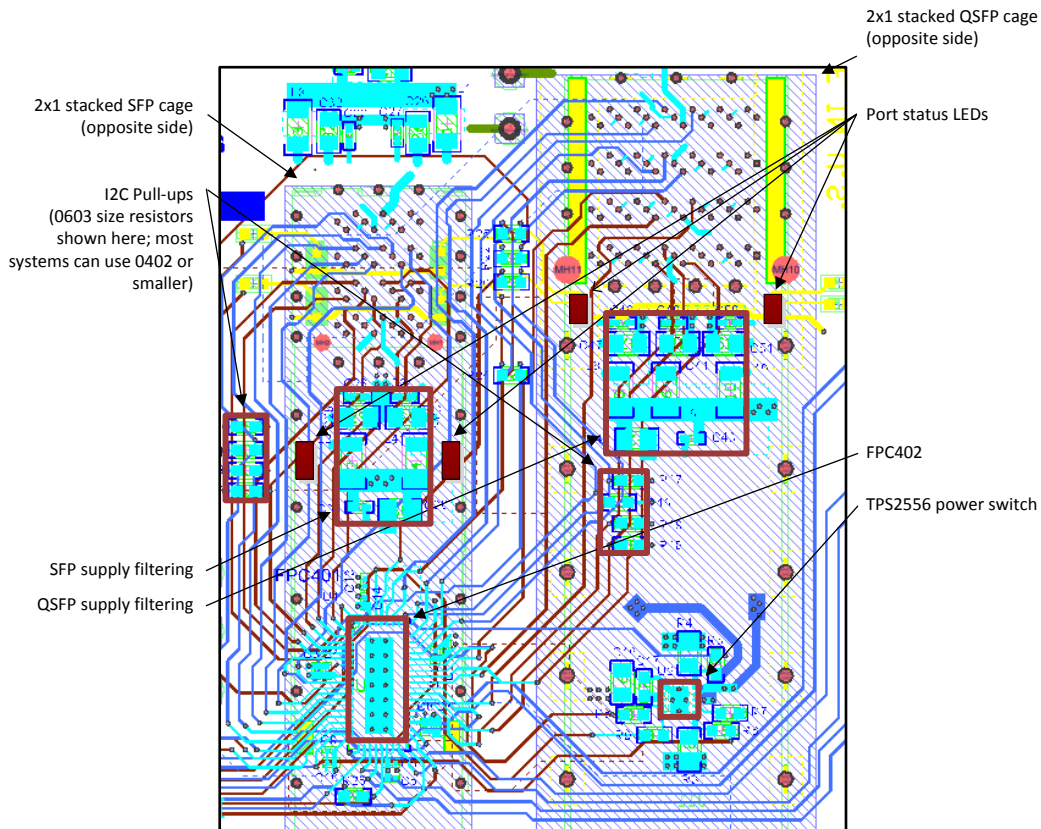
Figure 11-1. Layout Example
