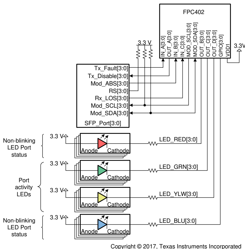
Figure 8-2. Example Configuration for Driving Four LEDs Per Port
