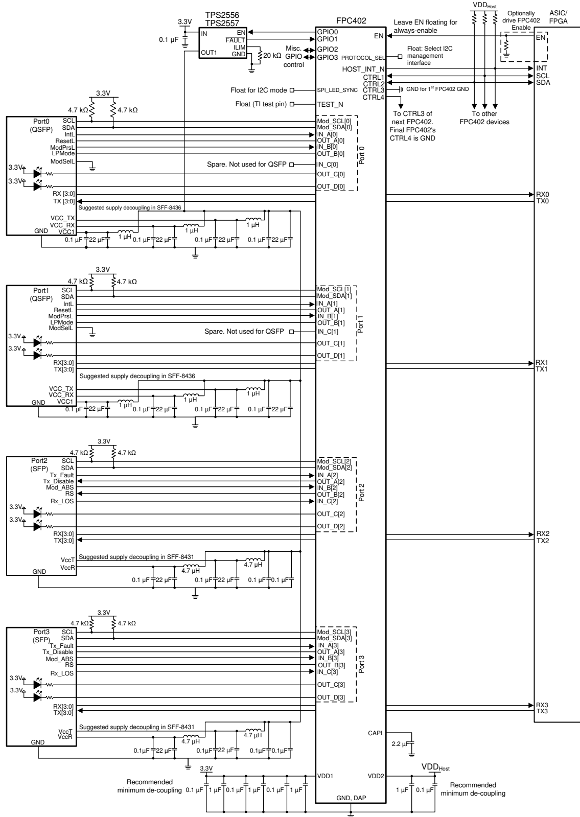
Figure 9-3. SFP/QSFP Application Schematic
