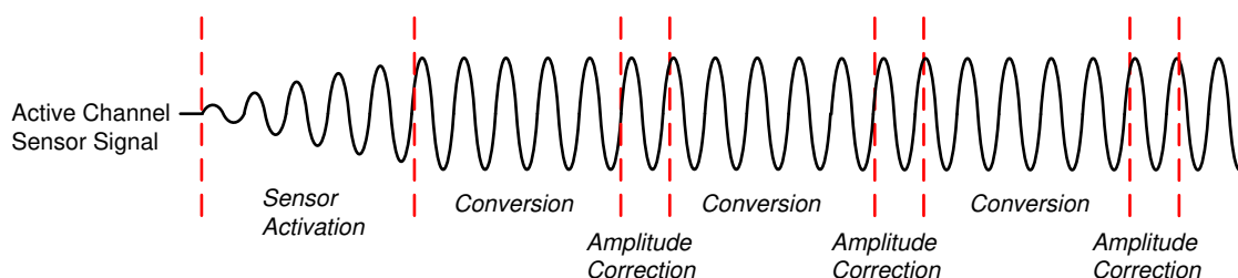
Figure 6-5. Single-Channel Mode Sequencing
