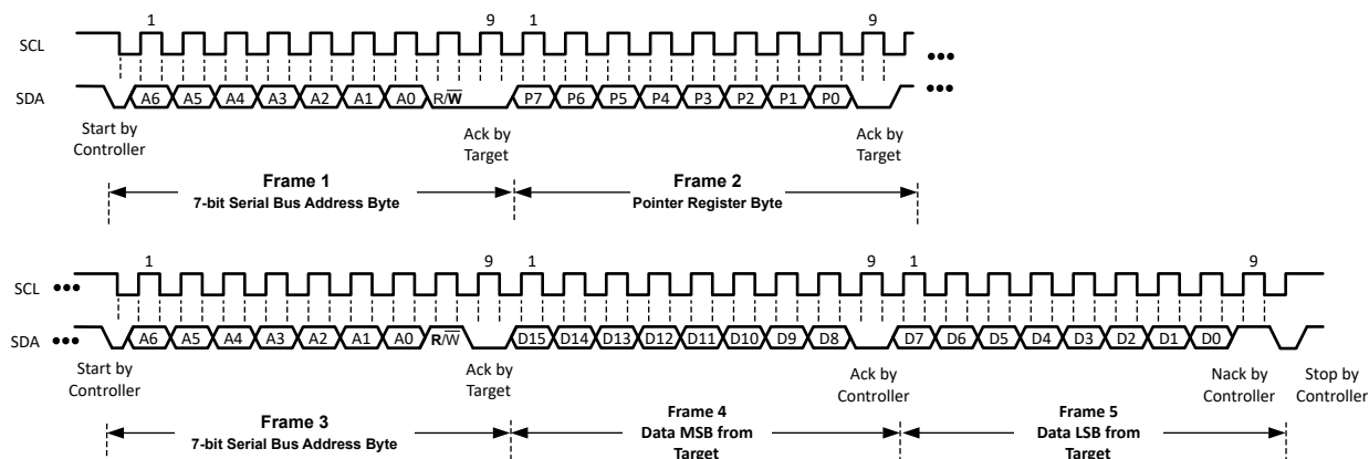
Figure 6-5. Read Frame
