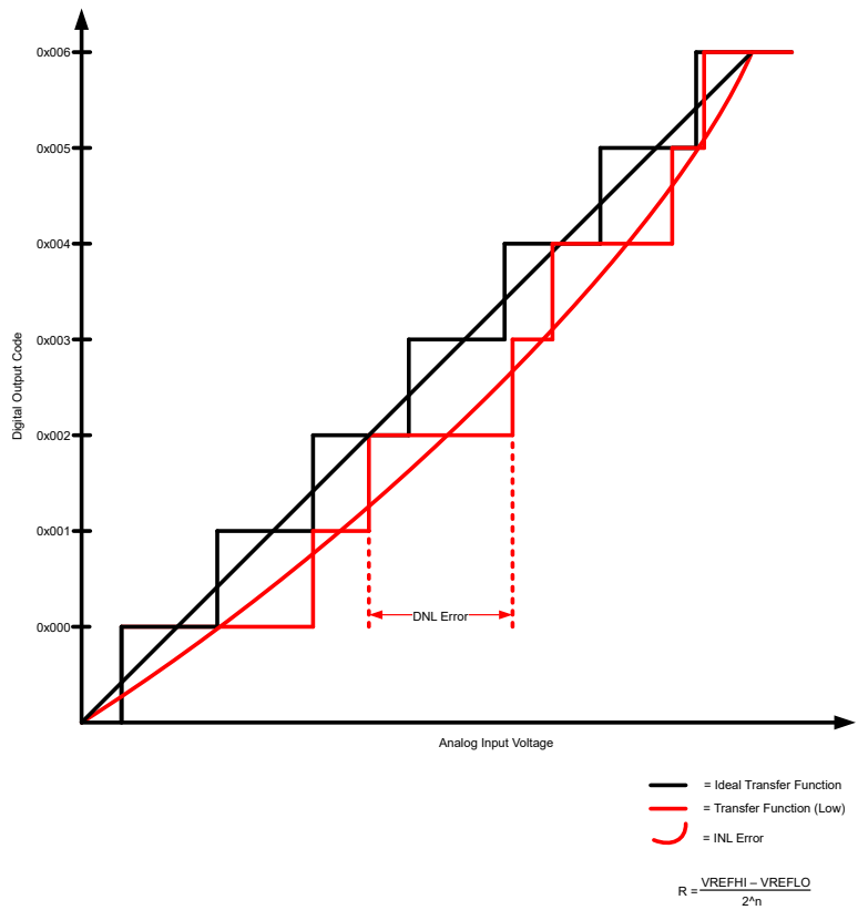
Figure 6-38. ADC INL and DNL
