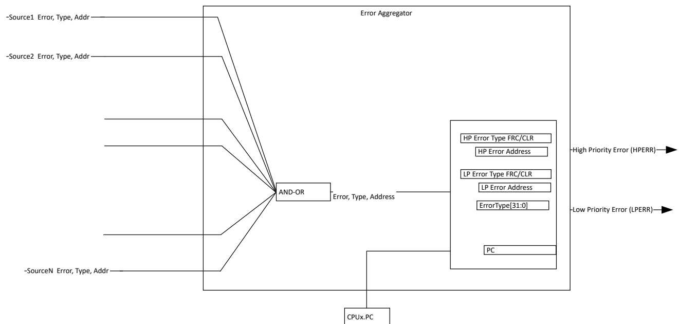
Figure 7-4. Error Aggregator Block Diagram
