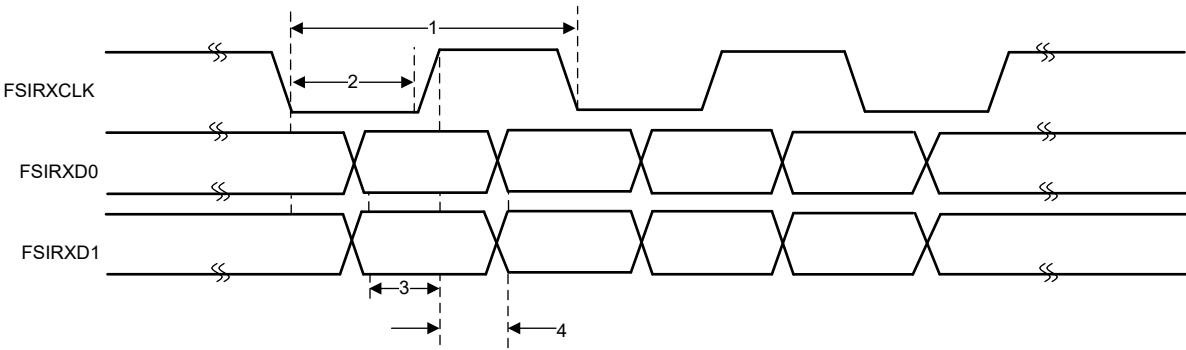
Figure 6-80. FSIRX Timings
