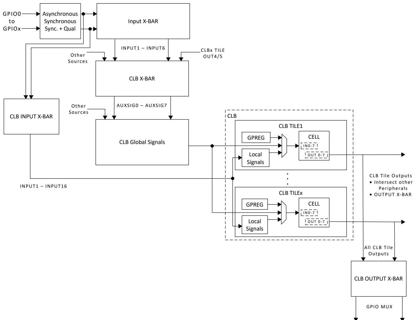
Figure 7-22. GPIO to CLB Tile Connections
