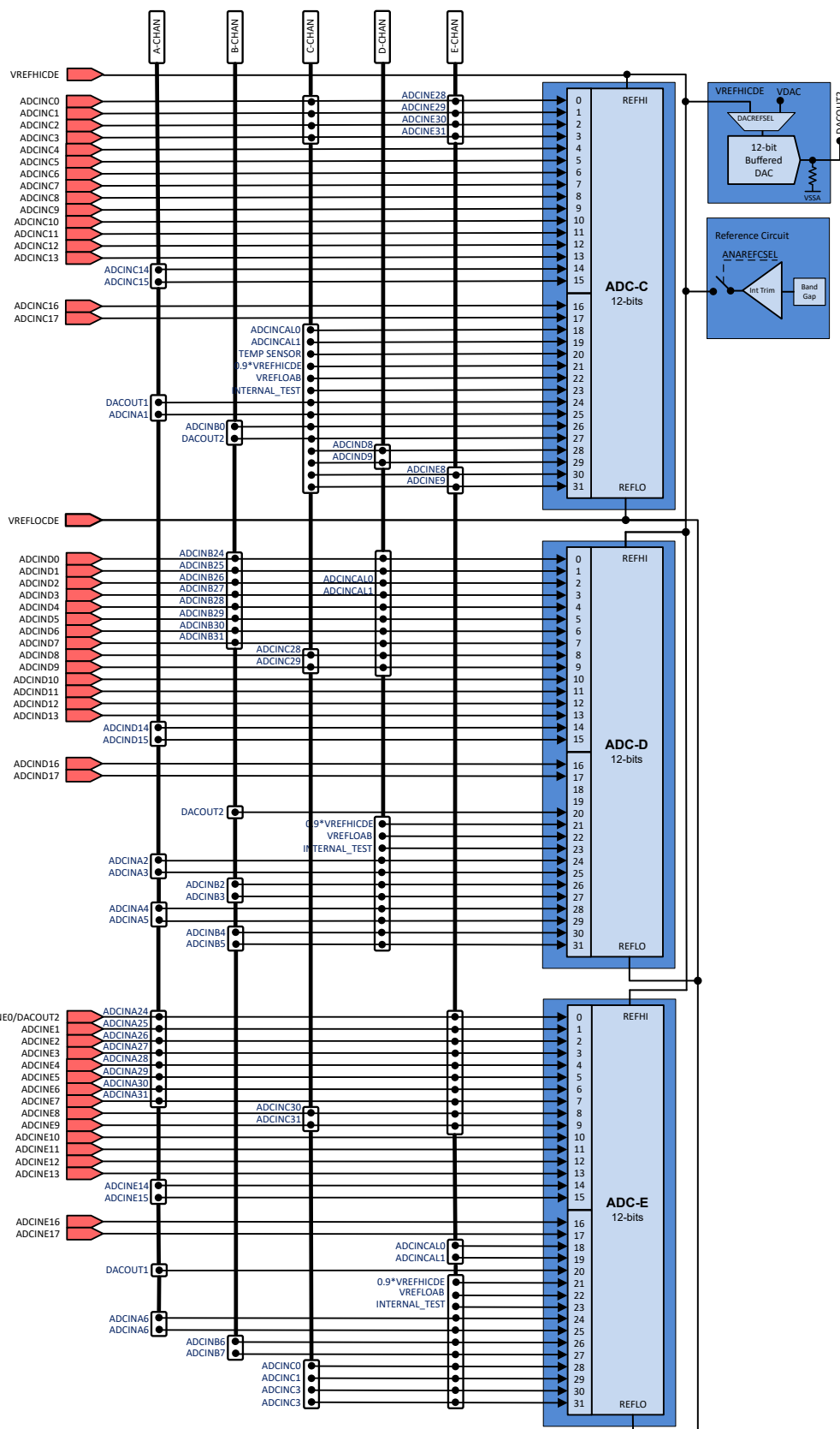
Figure 6-33. Analog Subsystem Block Diagram (ADC C, ADC D and ADC E)
