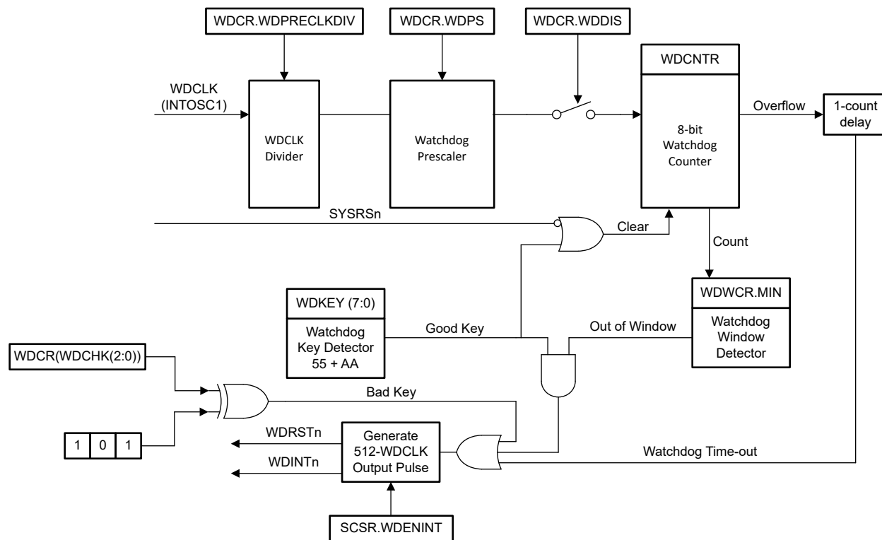
Figure 7-21. Windowed Watchdog
