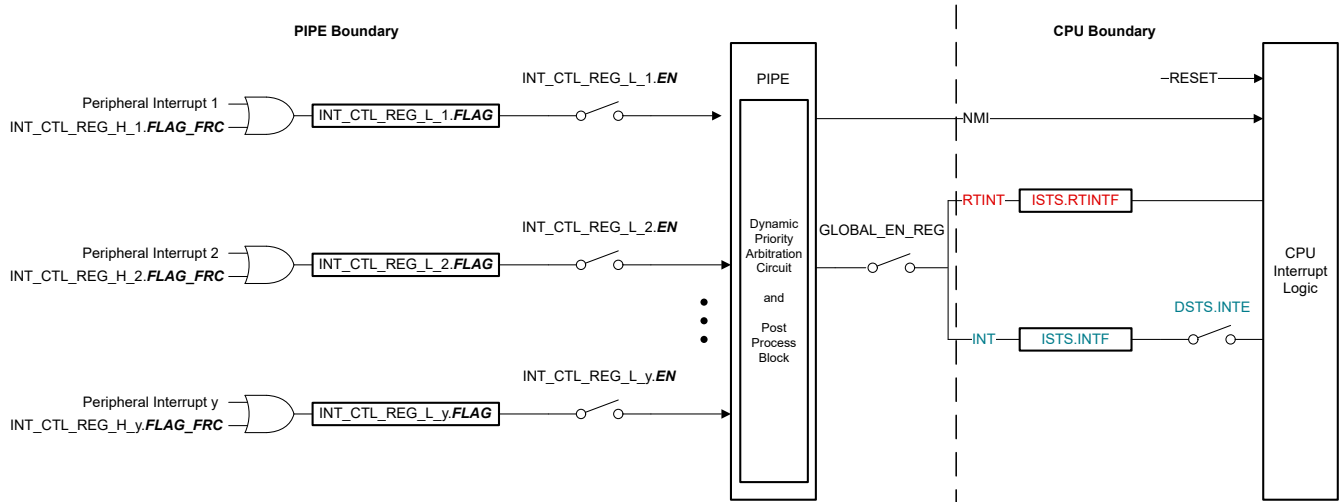
Figure 7-15. Interrupt Propagation
