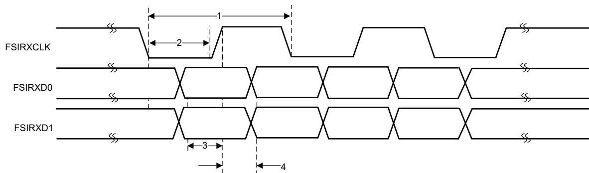
Figure 6-72. FSIRX Timings
