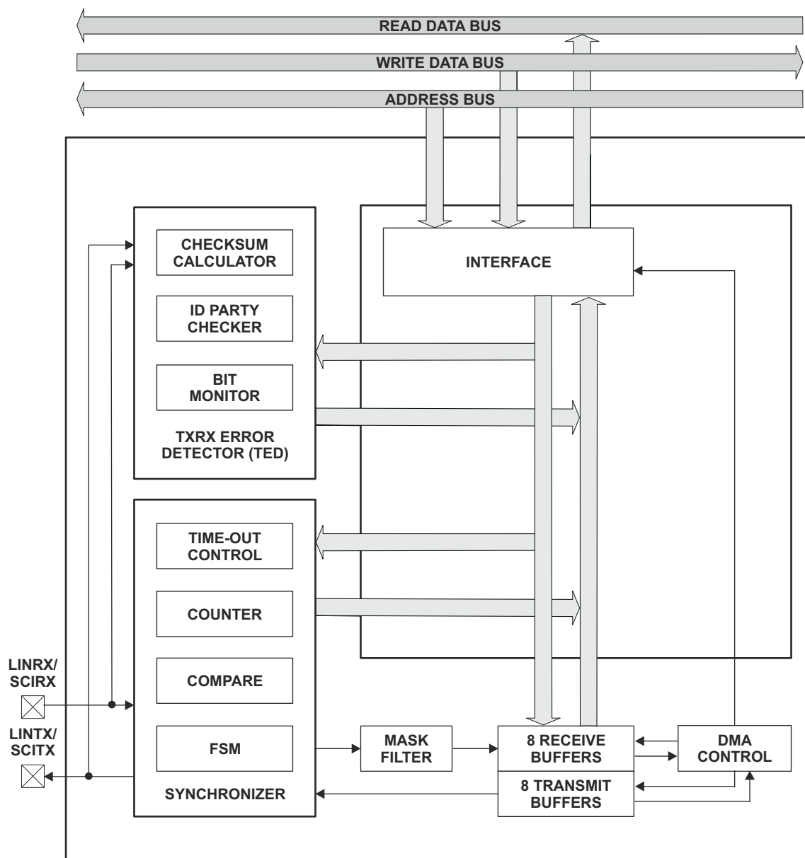
Figure 6-82. LIN Block Diagram
