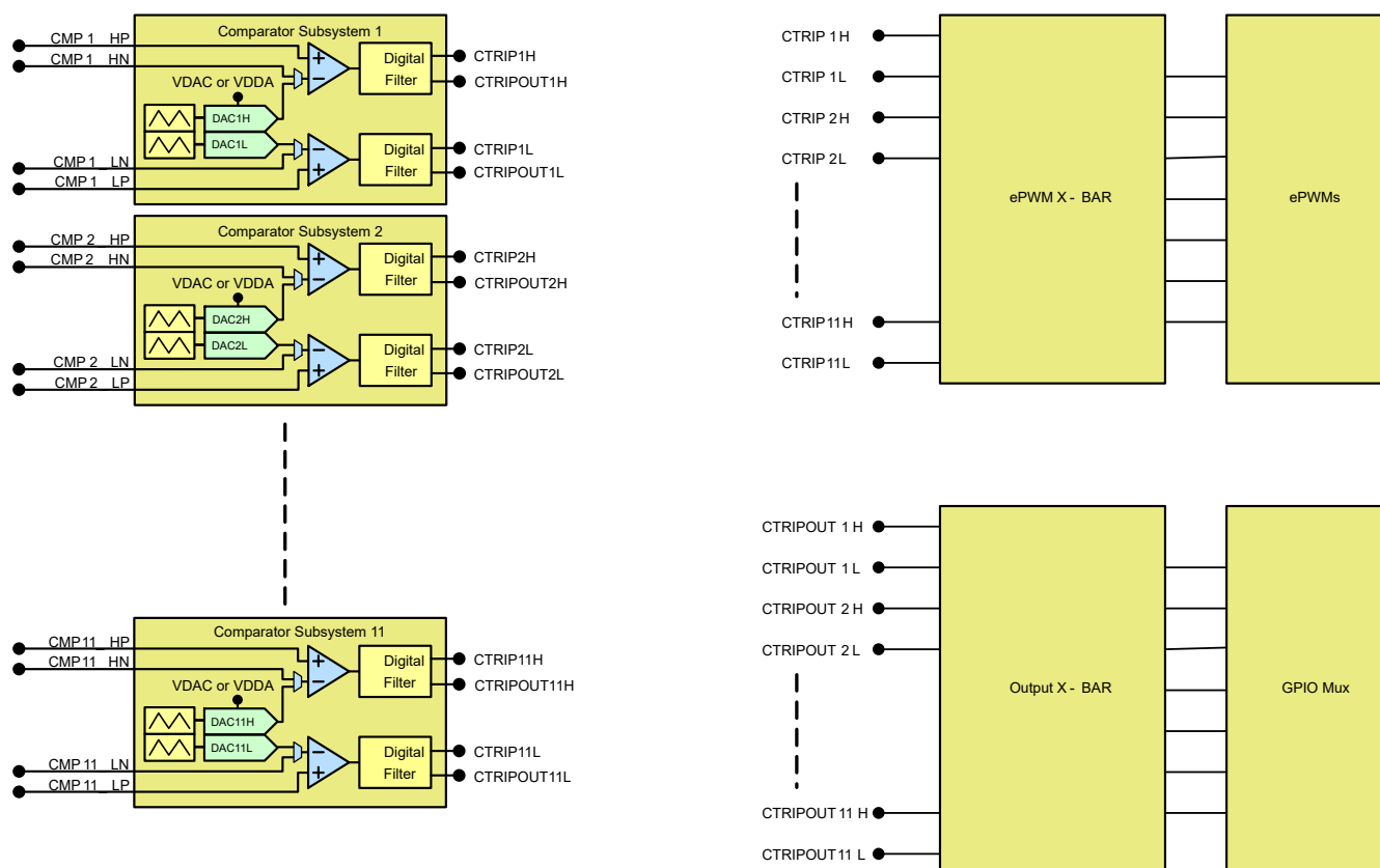
Figure 6-45. CMPSS Connectivity
