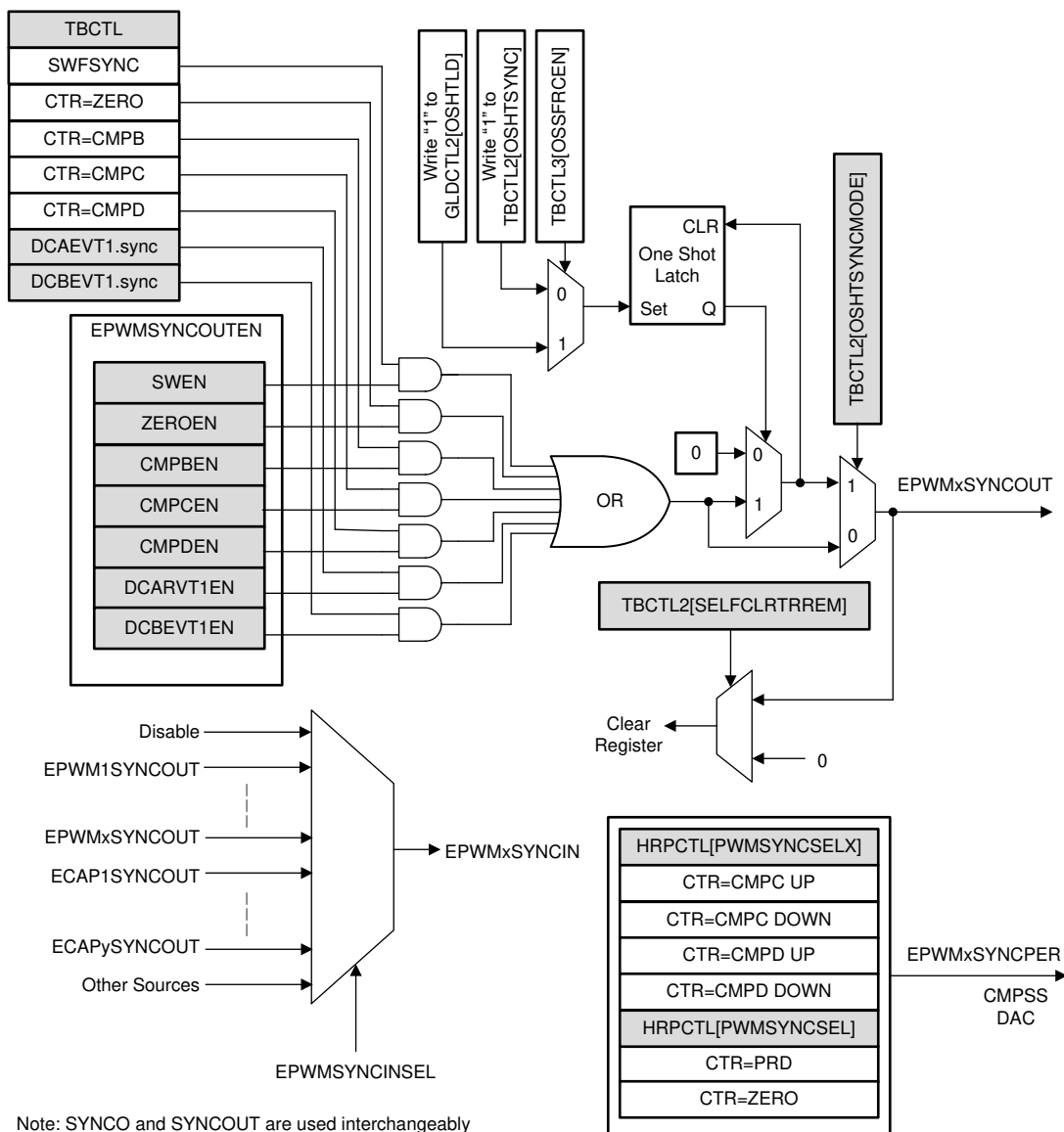
Figure 6-60. Synchronization Chain Architecture
