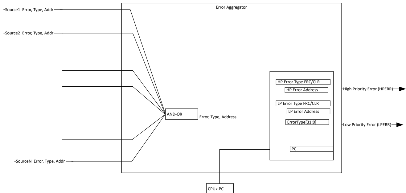
Figure 7-3. Error Aggregator Block Diagram
