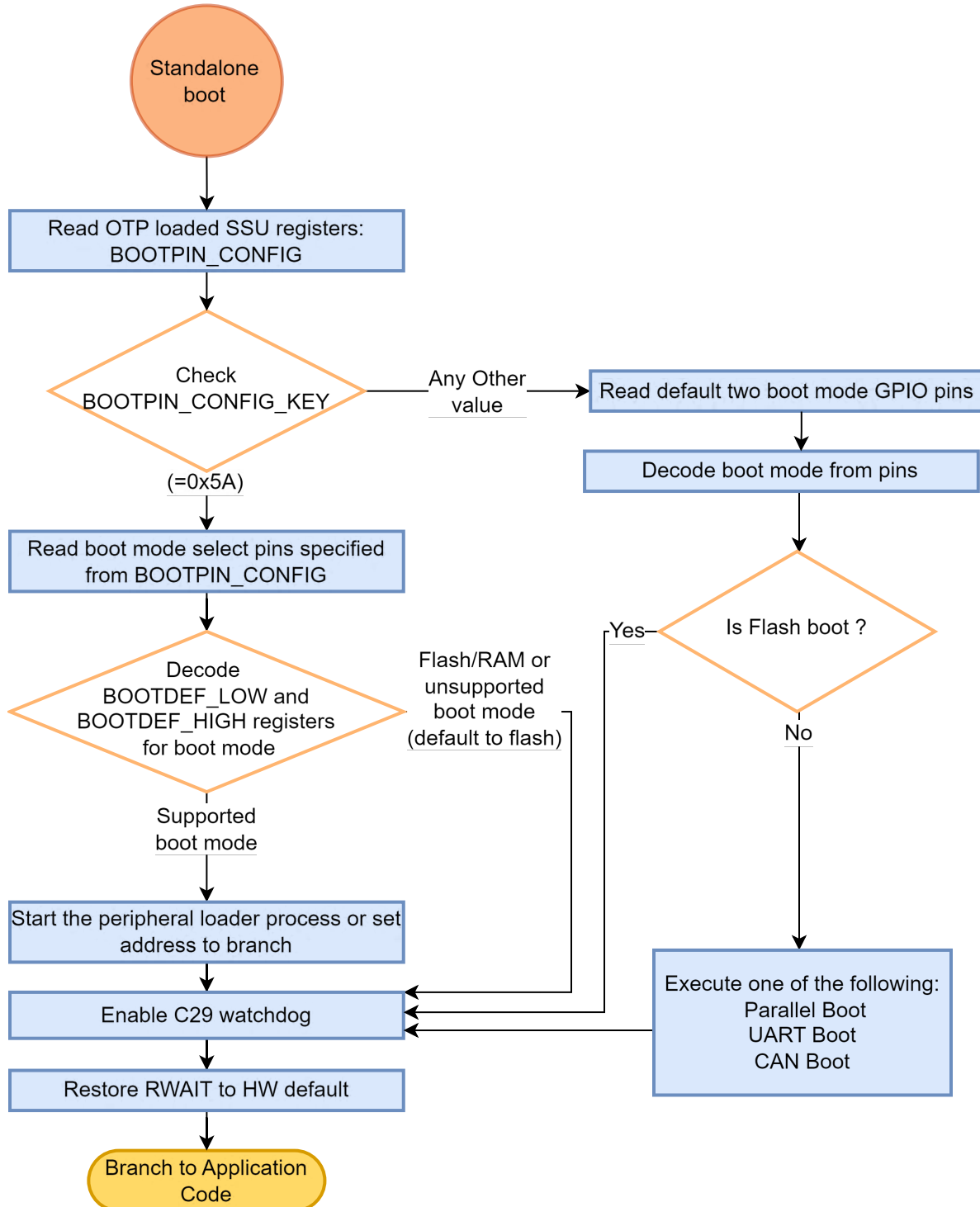
Figure 7-10. Stand-alone Boot Flow
