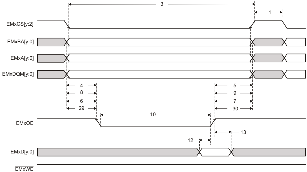
Figure 6-28. Asynchronous Memory Read Timing
