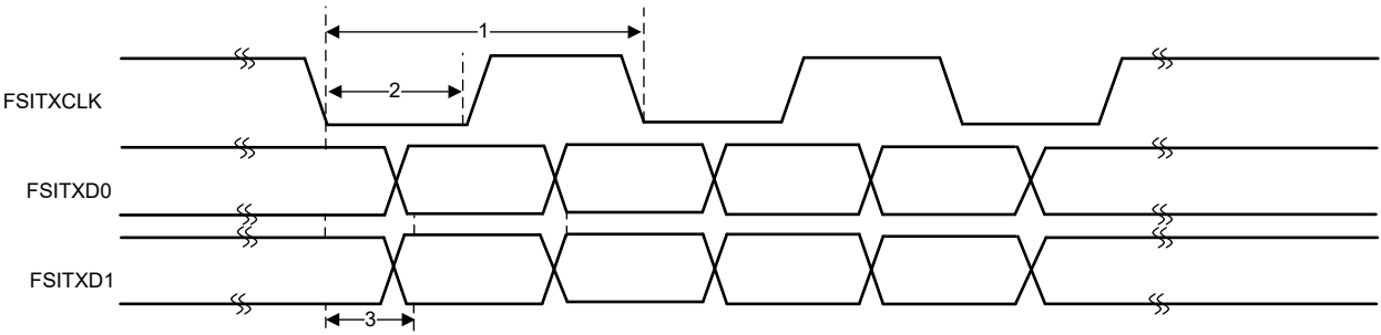
Figure 6-69. FSITX Timings
