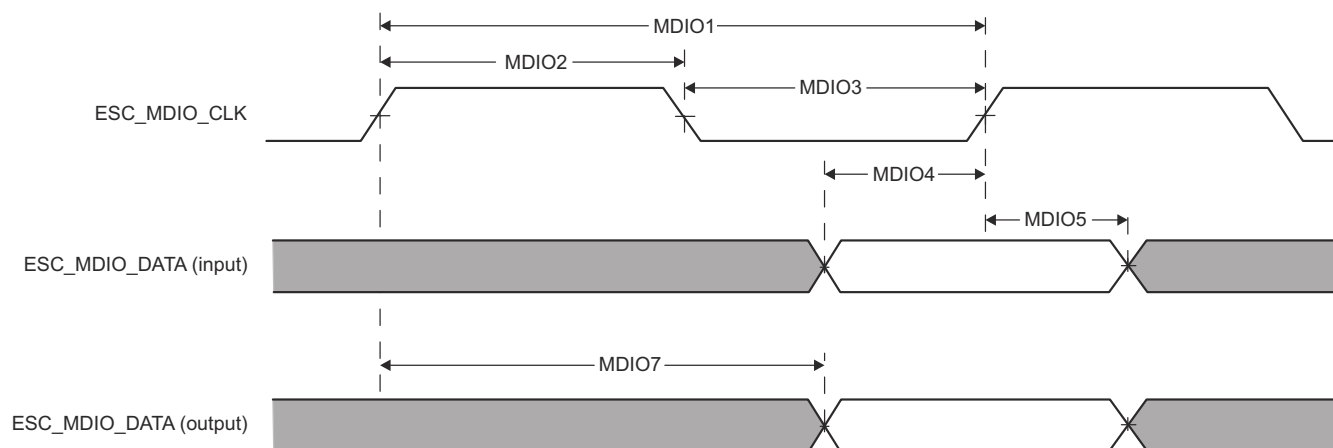
Figure 6-88. EtherCAT MDIO Timing Diagrams
