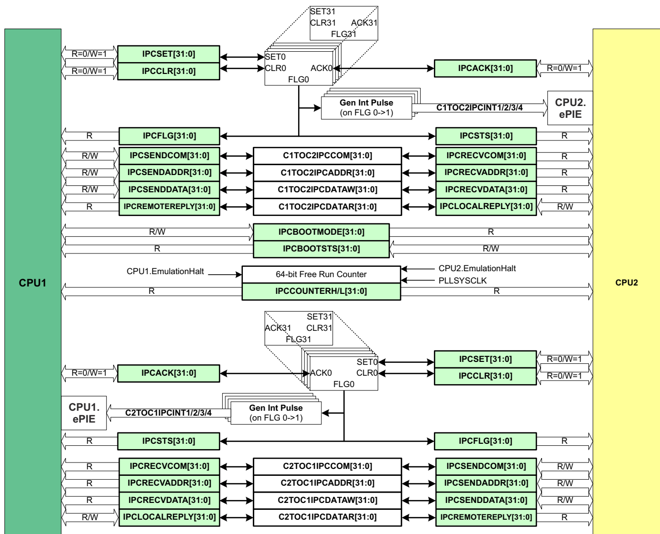
Figure 7-4. IPC Architecture
