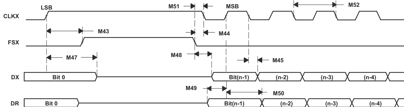
Figure 6-71. McBSP Timing as SPI Master or Slave: CLKSTP = 10b , CLKXP = 1
