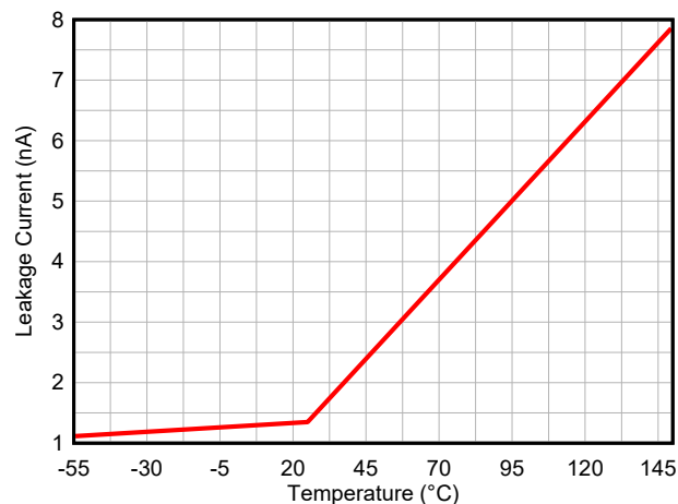
Figure 5-3. Leakage Current vs Temperature
