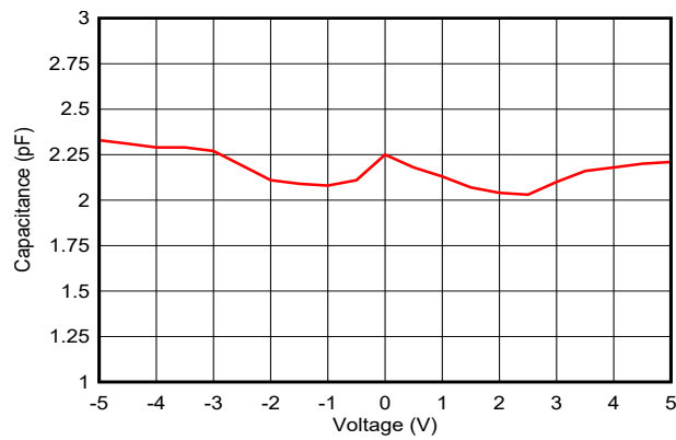
Figure 5-1. Capacitance vs. Bias Voltage
