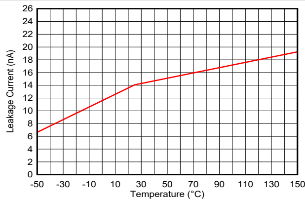
Figure 5-3. Leakage Current vs. Temperature
