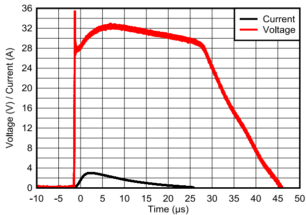
Figure 5-5. 8/20µs Surge Response
