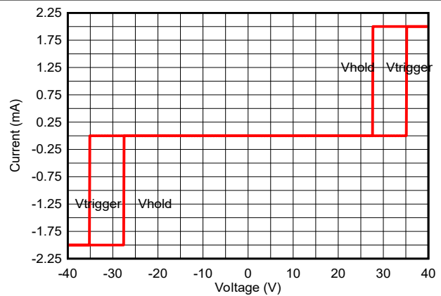
Figure 5-4. DC-IV Curve
