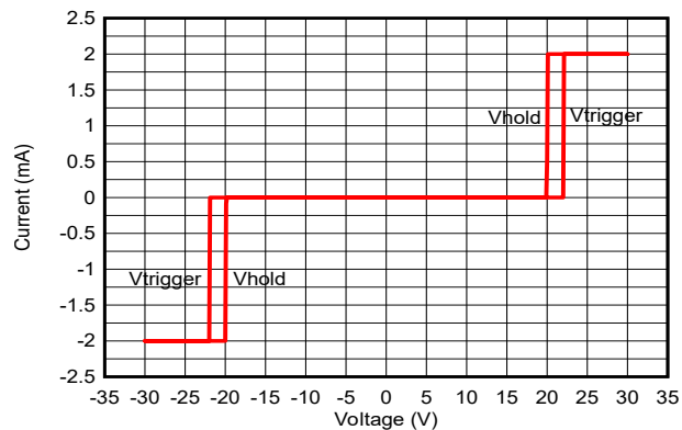
Figure 5-2. DC I-V Curve
