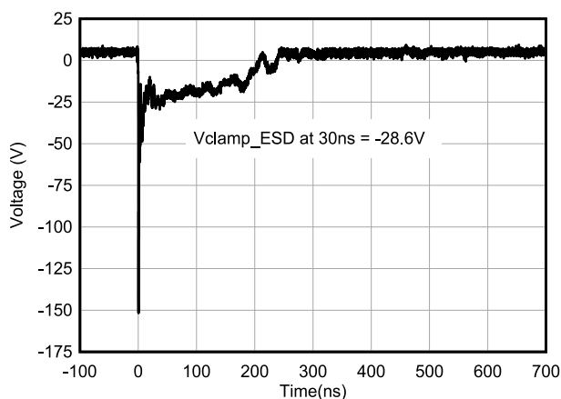
Figure 8-3. -8-kV Clamped IEC Waveform
