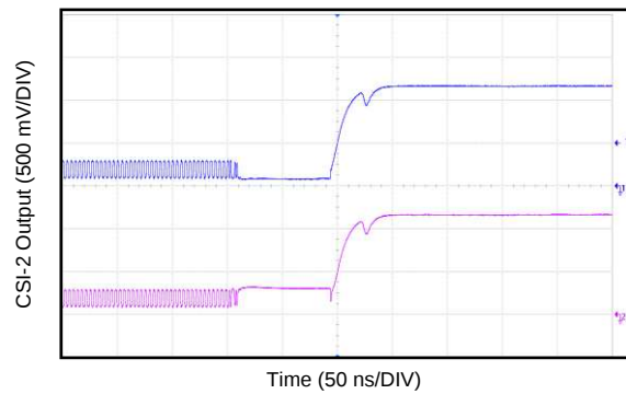
Figure 16. CSI-2 D0± End of Transmission
