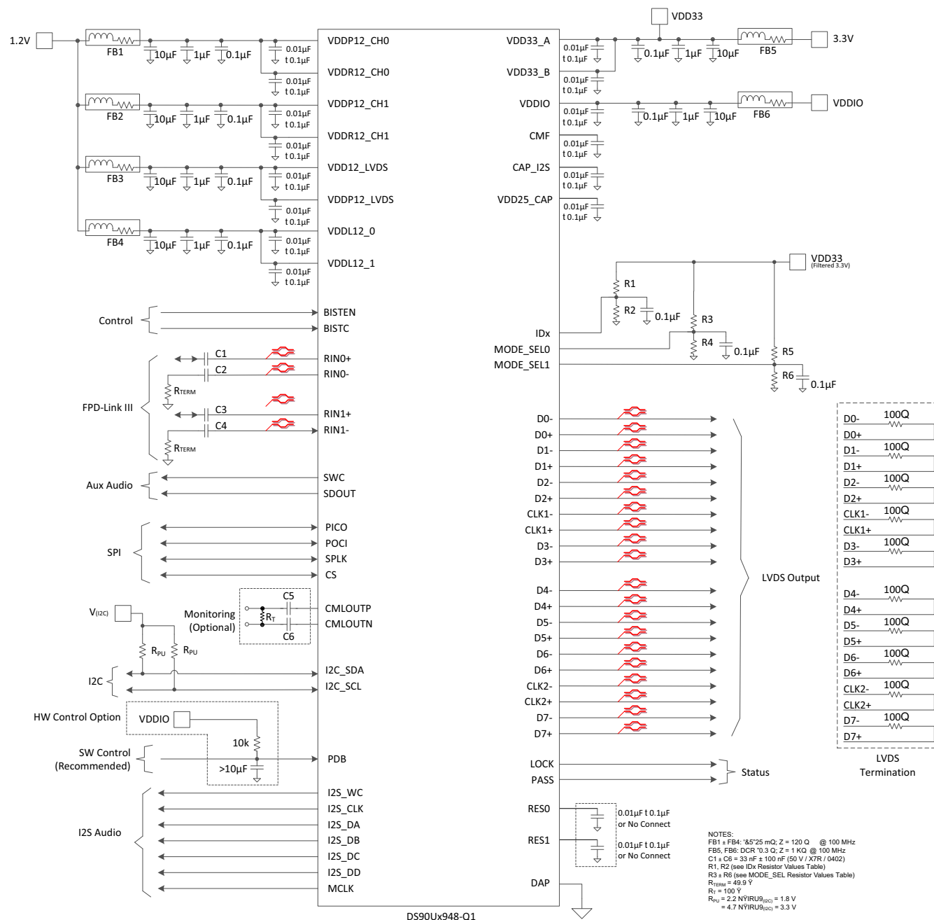
Figure 8-1. Typical Connection Diagram (Coax)
