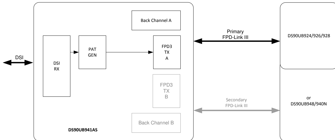
Figure 8-19. Single-Link, 1:1 Mode
