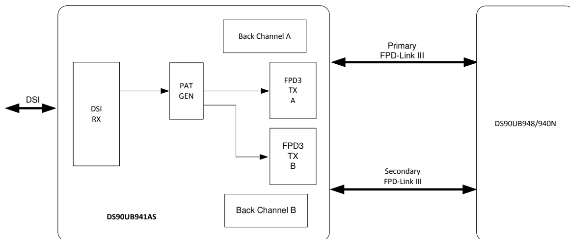
Figure 8-20. Dual-Link, 1:2 Mode
