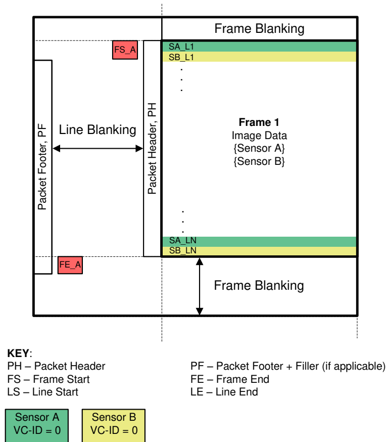
Figure 7-21. Line-Interleave Format
