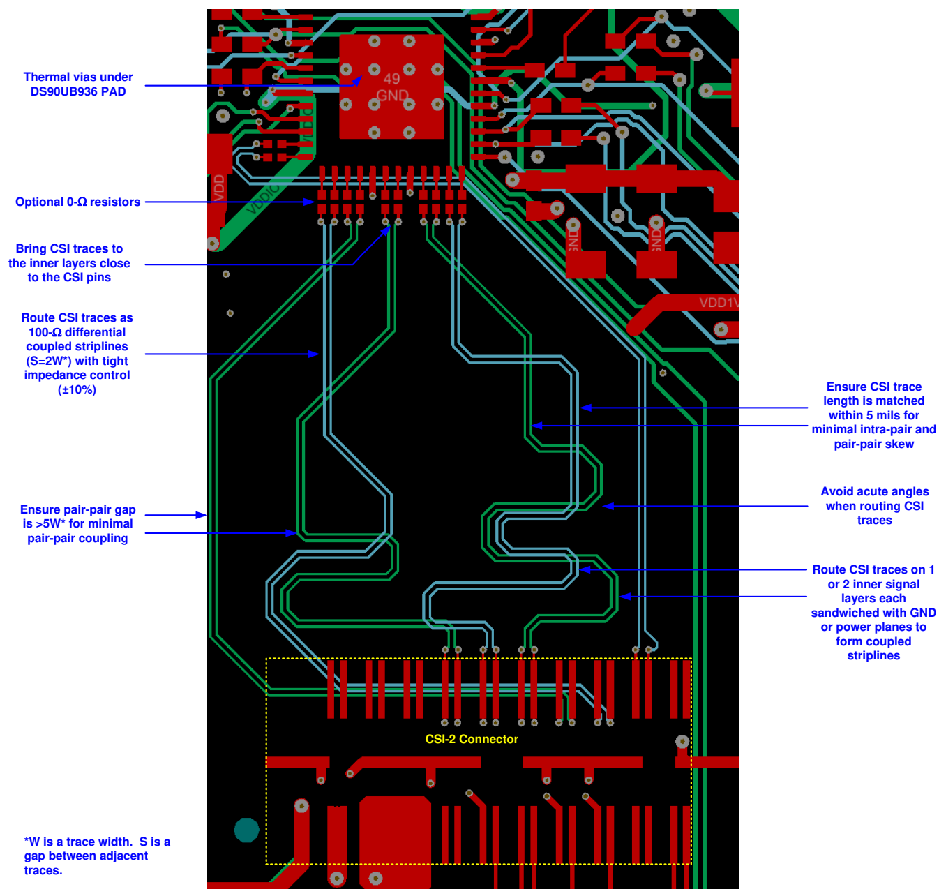
Figure 10-3. DS90UB936-Q1 PCB Layout Example: CSI-2 Traces
