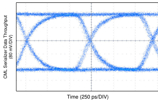
Figure 8-6. Coax Eye Diagram at 1.4-Gbps Line Rate (100-MHz Pixel Clock, 10-bit Mode) from Serializer Output (DOUT+)
