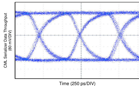
Figure 8-7. Coax Eye Diagram at 1.87-Gbps Line Rate (100-MHz Pixel Clock, 12-bit Mode) from Serializer Output (DOUT+)
