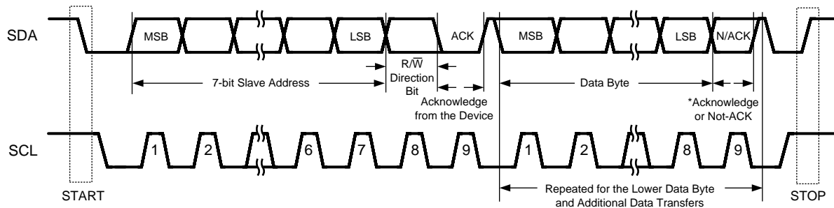
Figure 26. Basic Operation
