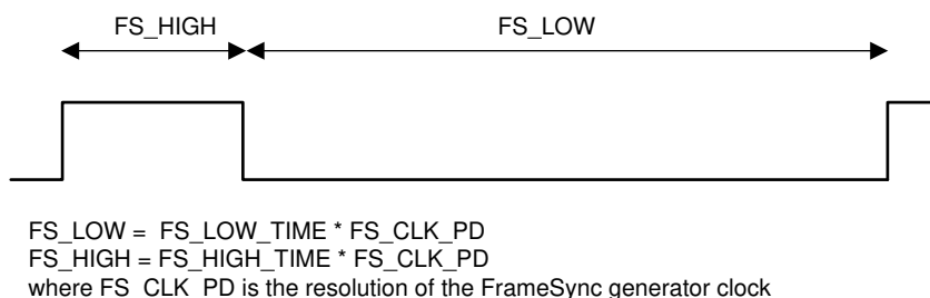
Figure 7-12. Internal FrameSync Signal
