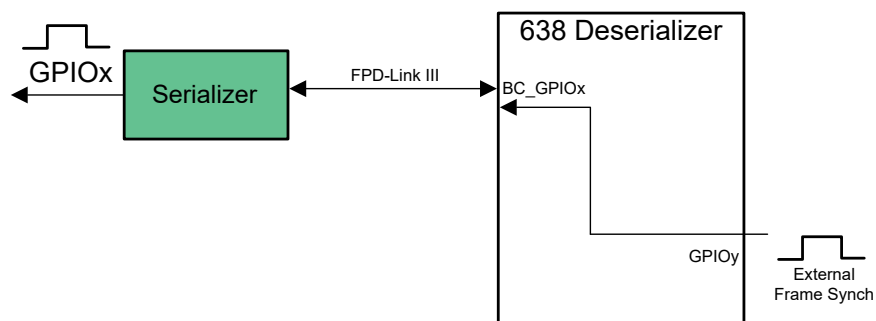
Figure 7-10. External FrameSync
