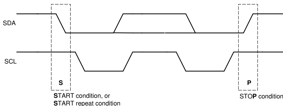
Figure 7-14. START and STOP Conditions
