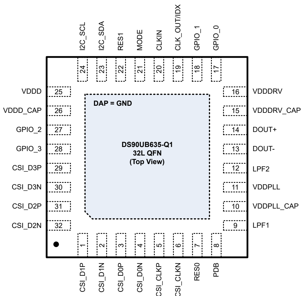
Figure 5-1. RHB Package 32-Pin VQFN Top View
