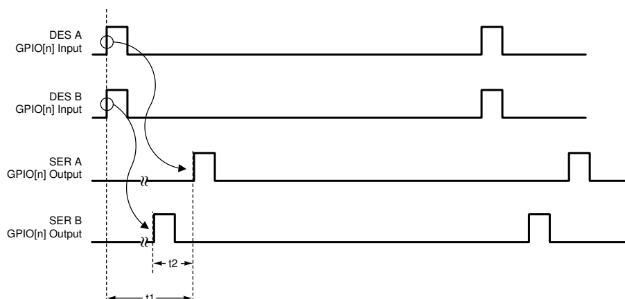
Figure 7-2. GPIO Delta Latency
