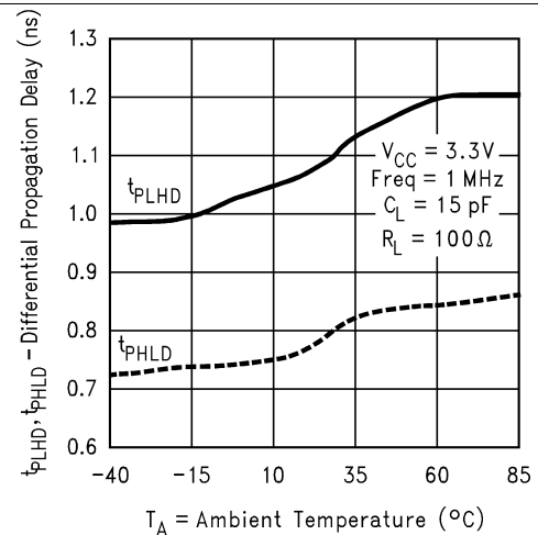
Figure 10. Differential Propagation Delay vs Ambient Temperature
